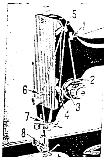
Fig. 14. Upper Threading.
