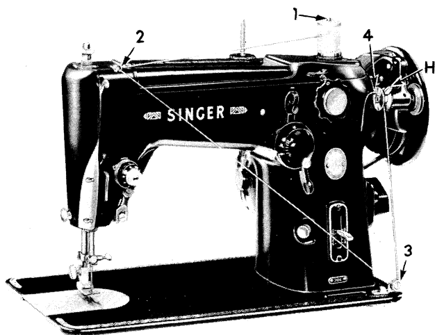
Fig. 8. To Wind the Bobbin.
