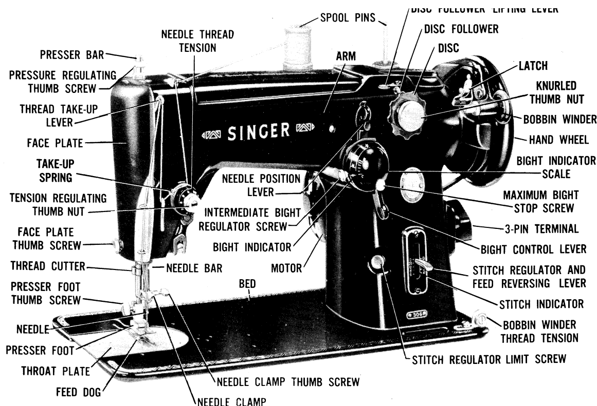
Fig. 40. Names of Principal Parts of Machine 306K25.
