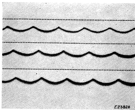
Fig. 104. Scalloped Tucks.
