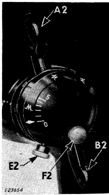
Fig. 41. Machine Set for Straight Stitching with Limit Screws Locked.
