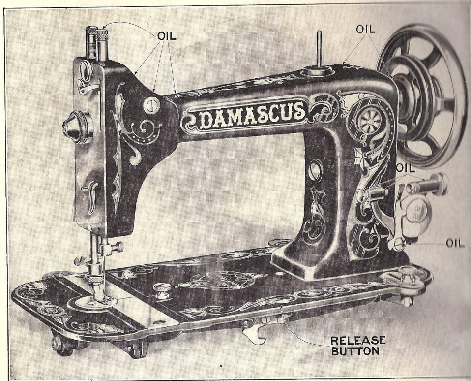
Figure 2. The arrows show the location of the oil holes where a drop of oil is needed. There is an oil hole in the top of the needle bar cap and three oil holes which distribute the oil to the sewing head. There are two oil holes on the arm near the balance wheel and one on the automatic bobbin winder.
