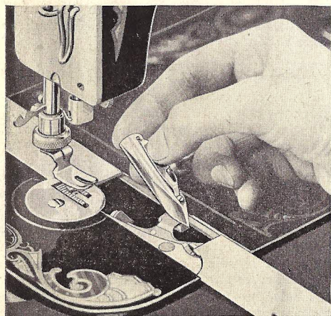
Figure 8. Turn the machine until the shuttle carrier is in the forward position, place the point of the shuttle between the shuttle race and the carrier and drop the shuttle into place.
