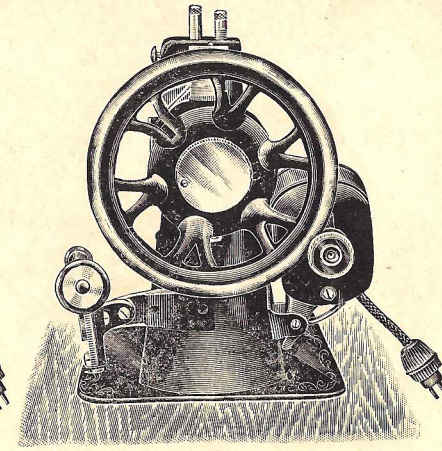
FIG. 2—Ready to sew. Bobbin winding mechanism away from hand wheel.
