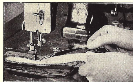
Figure 17. The binding fills the scrolls of the binder and the cloth is inserted between the scrolls.
