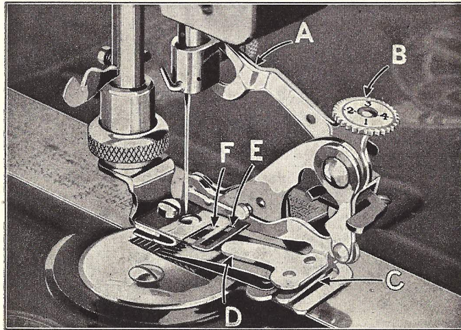
Figure 19. Attach the ruffler to the presser bar in place of the presser foot with the forked lever A astride the screw of the needle clamp.
