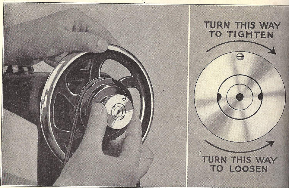
Figure 5. To release the sewing mechanism, hold the hand wheel with your left hand and turn the friction nut with your right hand. The picture at the right shows the direction to turn the brake button to tighten or loosen it. It is only necessary to turn the brake button about one half turn.
