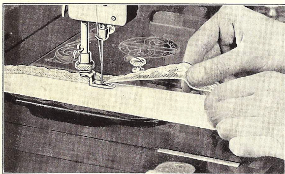
Figure 15. Guide the cloth with the left hand so the mouth of the hemmer is kept just full. The right hand guides the lace into the slot of the hemmer so the needle will pierce it.
