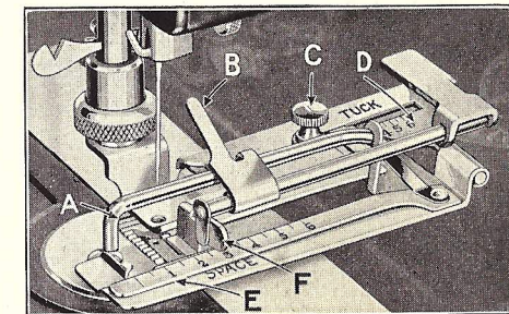
Figure 18. By loosening the set screw C the scales of the tucker can be adjusted for tuck and space.
