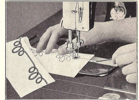
Figure 21. Sew on the wrong side of the cloth and feed the braid through the under-braider slide.
