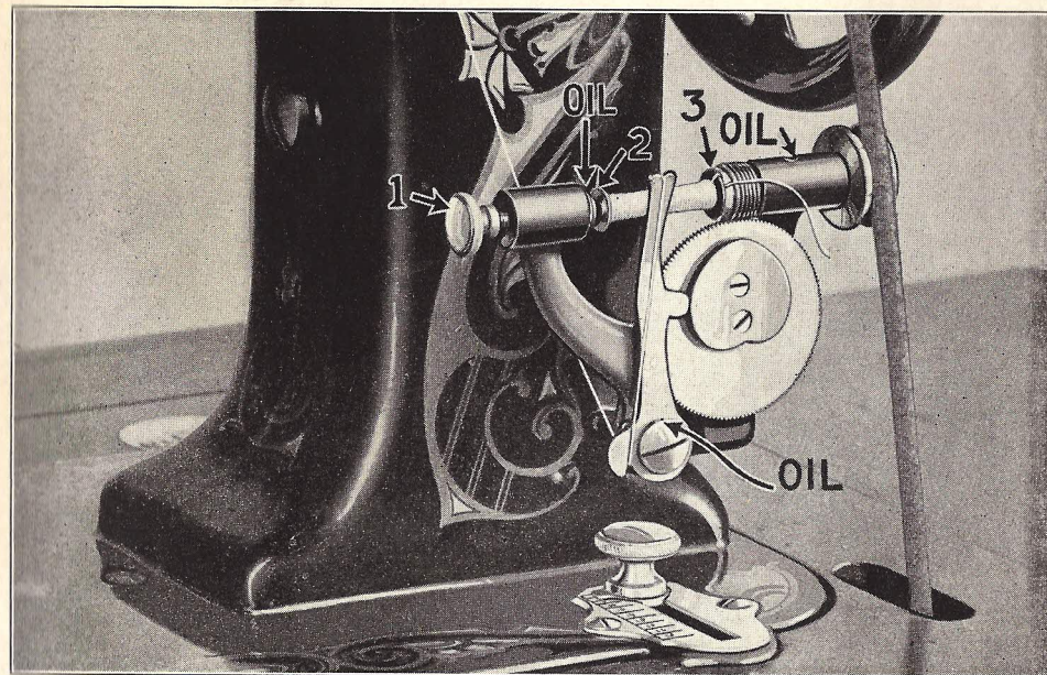
Figure 6. This shows how the automatic bobbin winder is turned into position with the small pulley in line with the belt pulley of the machine. Notice how the end of the thread is caught between the brass end of the bobbin and the socket (3) to hold the thread as the bobbin starts winding.
