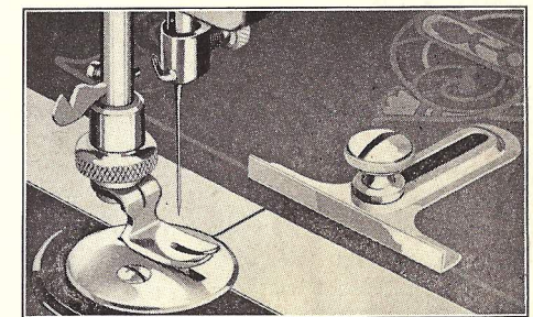
Figure 23. The adjustable cloth guide thumb screw is fastened to the bed plate of the machine before it is shipped. This attachment enables you to sew straight seams.
