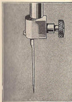
Figure 9. Insert the needle in the needle clamp with the flat side of the shank to the right as you sit facing the machine.
