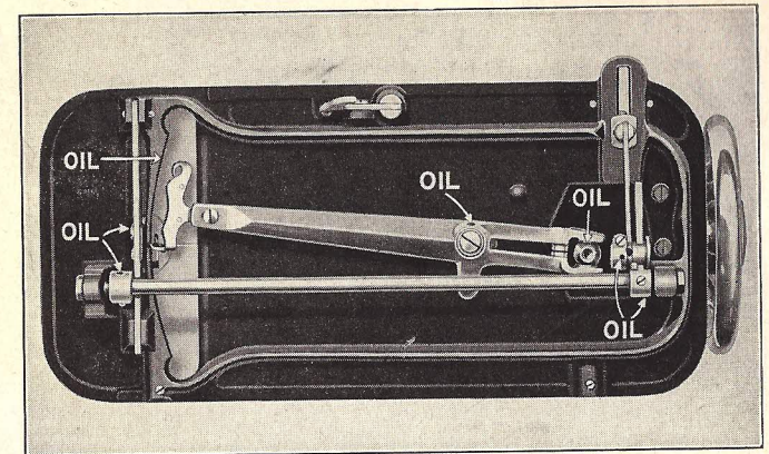
Figure 3. This shows the sewing head turned back on its hinges and the arrows indicate the points where oil is needed. A drop of oil at each point is sufficient and any surplus should be wiped away.
